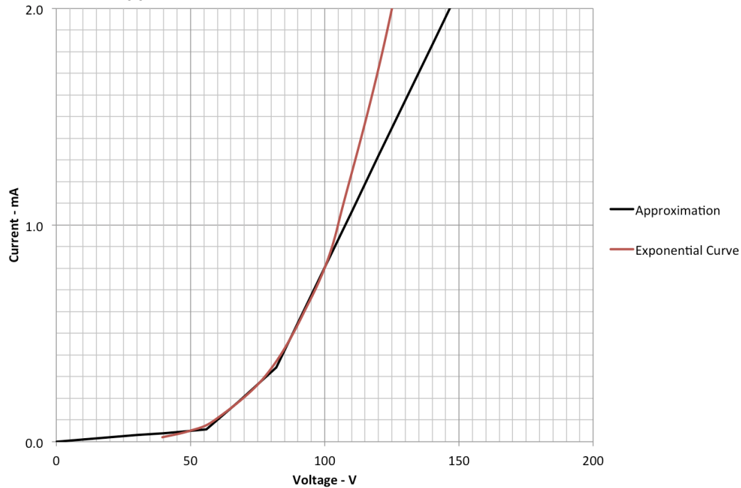
Approximation of Varistor with Zener Diodes and Resistors
